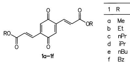
Scheme 1. Formula scheme of compounds 1a–1f
