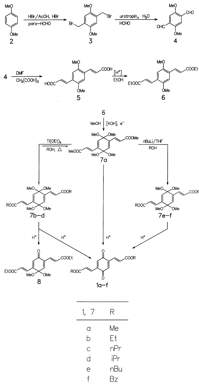
Scheme 2. Synthesis of the ( E,E )-2,5-bis(2-alkoxycarbonyl-ethenyl)-1,4-benzoquinones 1
