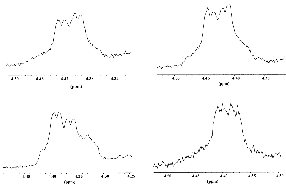
Figure 10. ^1\text{H} -NMR signals of the cyclobutane protons after irradiation of quinone 1c (top left), 1d (bottom left), 1e (top right) and 1f (bottom right)
