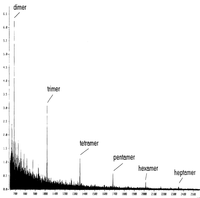
Figure 5. FAB-MS spectra of the quinone 1c after irradiation using filter A
