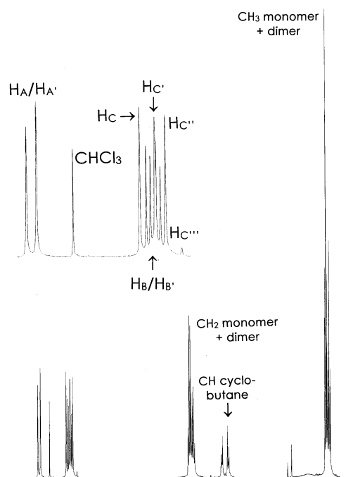
Figure 8. ^1\text{H} -NMR spectra of the quinone 1b after irradiation using filter B
