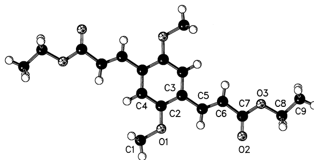
Figure 1. Molecular structure of compound 6 with labelling [14] : C2–C3 1.404(3), C2–C4 1.381(3), C3–C4' 1.393(3), C3–C5 1.469(3), C5–C6 1.300(3), C6–C7 1.479(3) Å
