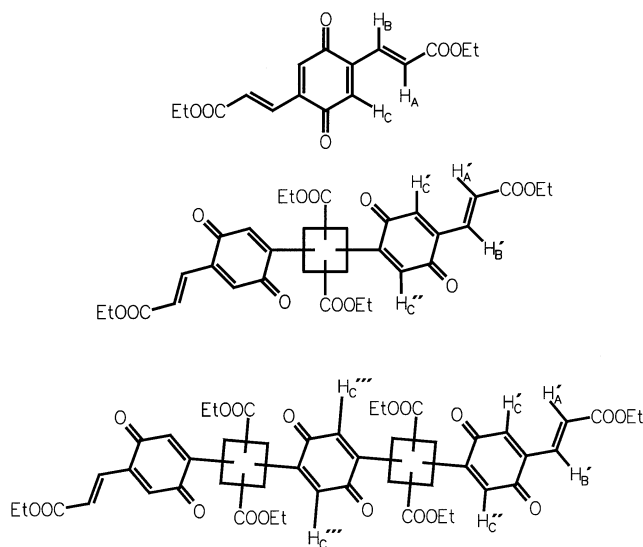
Scheme 3. Assignment of the ^1\text{H} -NMR and ^{13}\text{C} -NMR signals for the compounds 5 , 6 , 7a–7f and 1a–1f
