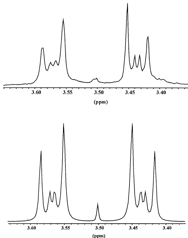
Figure 7. ^1\text{H} -NMR signals of the cyclobutane protons after irradiation of quinone 1b using filter B (top) and simulated ^1\text{H} -NMR spectra of a cyclobutane ring with \text{C}_2 symmetry
