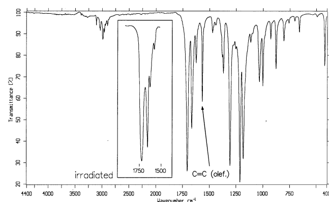
Figure 4. IR spectra of the quinone 1b before and after irradiation using filter B
