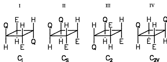
Figure 6. All possible configurations of cyclobutane ring systems generated by irradiation of trans double bonds in the solid state, trans/cis isomerization excluded
