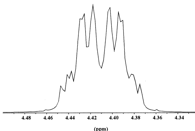
Figure 9. Simulated ^1\text{H} -NMR spectra of a cyclobutane ring with C_i symmetry
