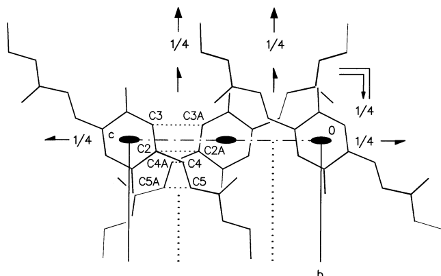
Figure 3. Packing arrangement of compound 1b
