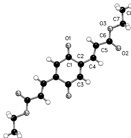
Figure 2. Molecular structure of compound 1b with labelling: C1–C2 1.502(12), C2–C3 1.332(11), C1–C3' 1.470(12), C2–C4 1.461(12), C4–C5 1.337(10), C5–C6 1.475(12) Å
